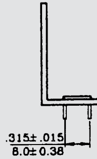
OPTION N FOUR GROUNDING BRACKETS (LOCKING TYPE)
