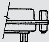
Option KJ With #4-40 Threaded Riveted Clinch Nuts And Jack Screws Assembled to Connector
